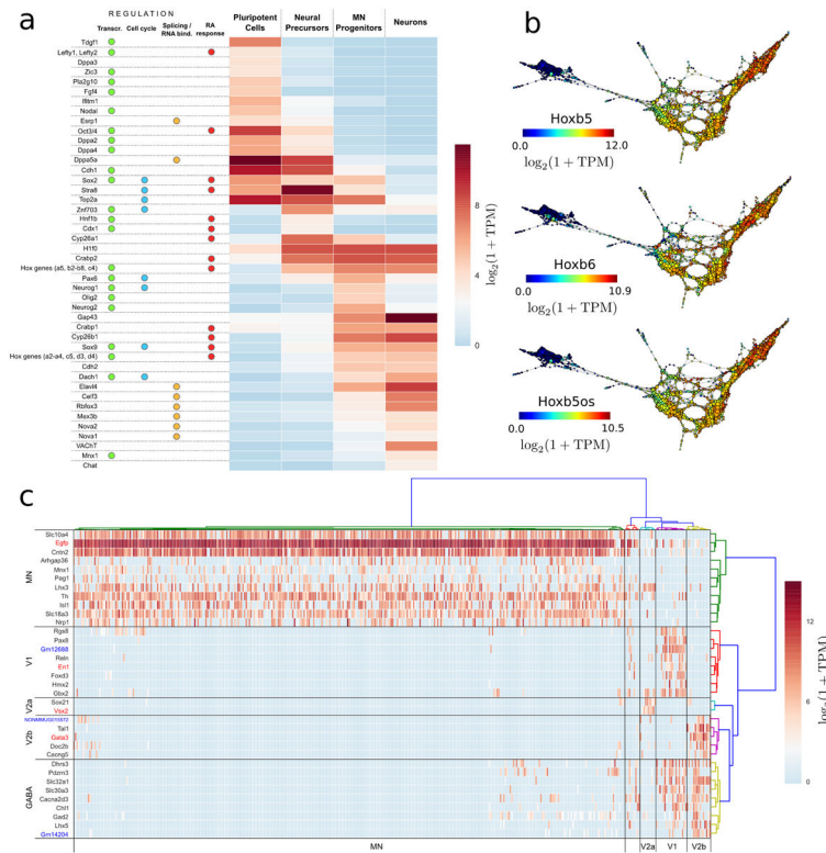
Figure 5. Differential gene expression in neurogenesis
