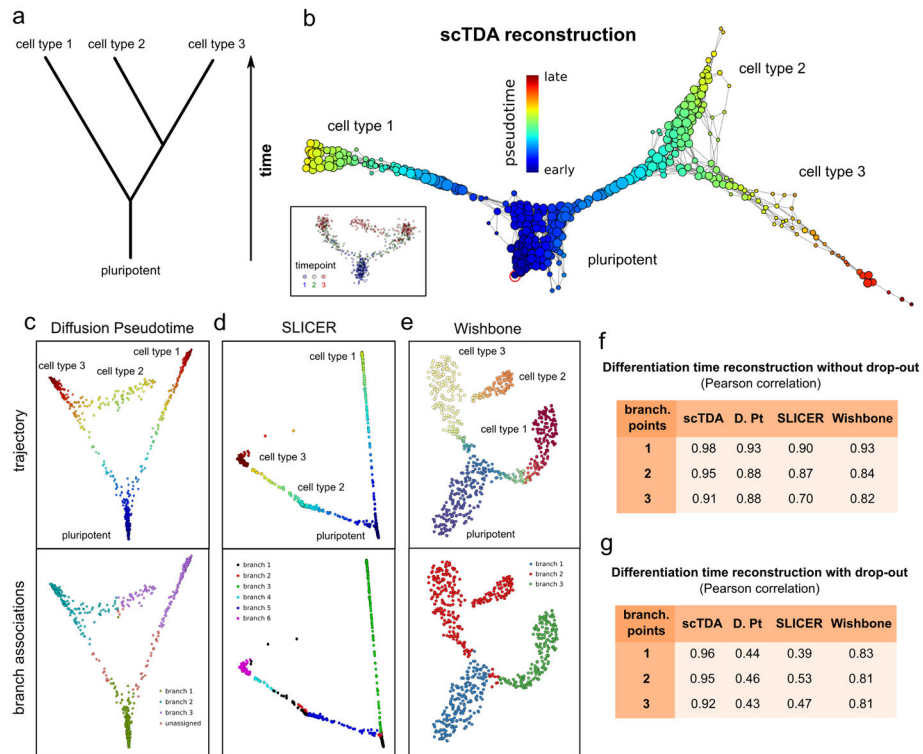
Figure 2. Comparison of algorithms for ordering cellular states
