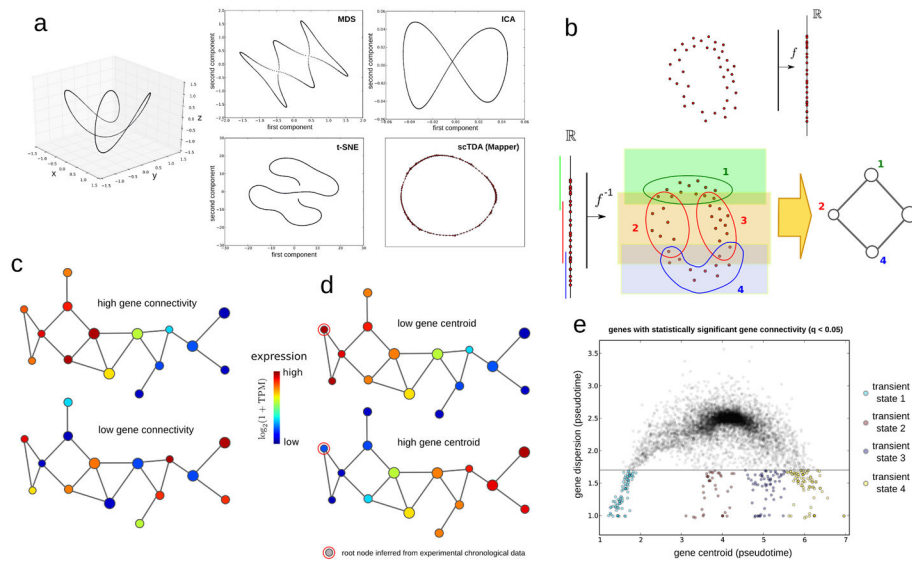
Figure 1. Topological analysis of longitudinal single-cell RNA-seq data
