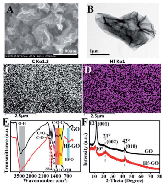
Fig. 2 (A) SEM image, (B) TEM image, (C and D) C and Hf EDS mappings of Hf-GO, (E) FTIR spectra, (F) XRD patterns of Hf-GO and GO.
