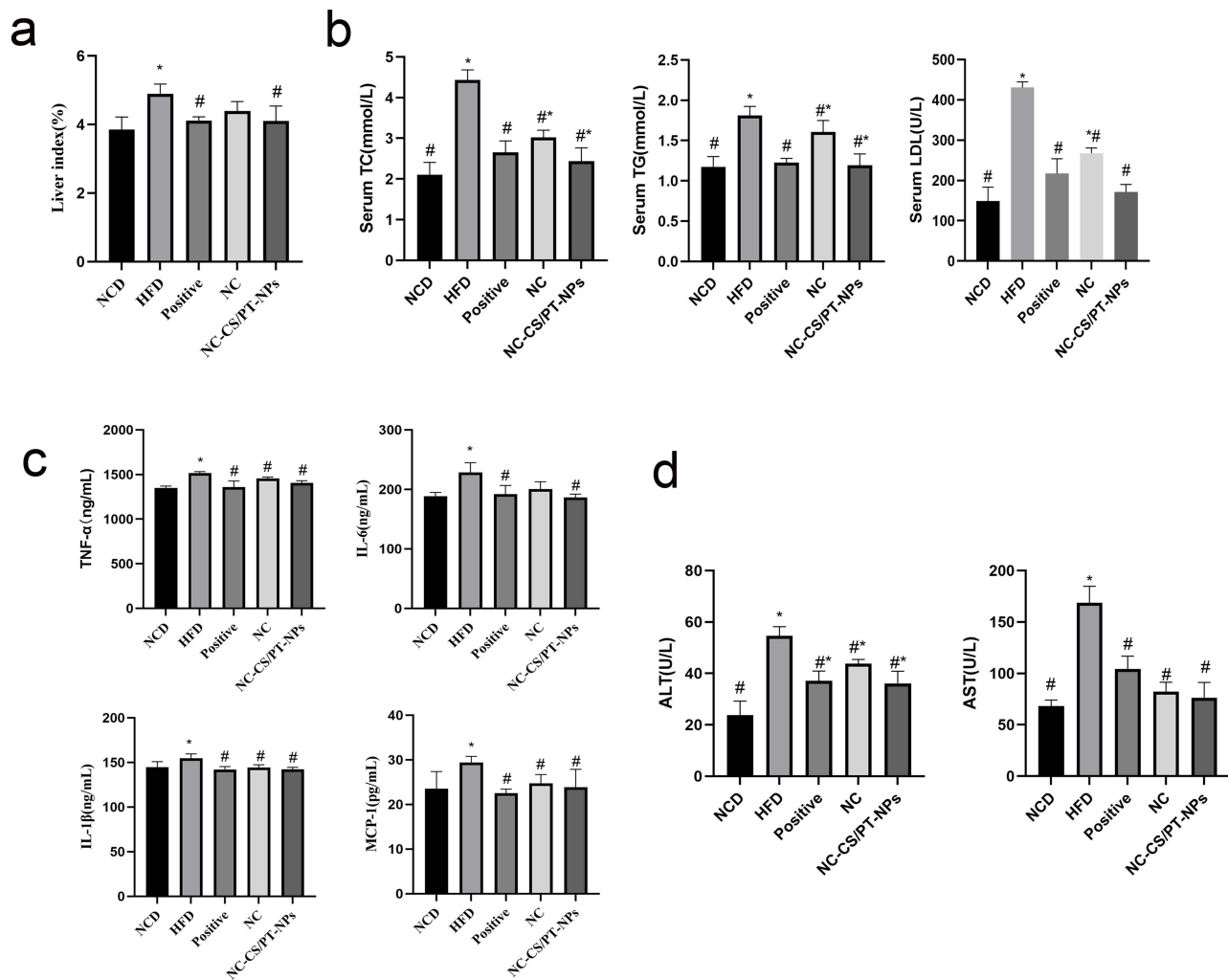
Figure 5 The Effect of NC-CS/PT-NPs on NAFLD Mice. (a) Liver Index of NAFLD Mice. (b) Serum TC, TG, LDL levels of mice in different groups. (c) TNF- \alpha , IL-6, IL- \beta , MCP-1 levels in liver tissues of mice. (d) Serum ALT, AST levels of mice in different groups. Compared with NCD group, * p < 0.05 ; compared with HFD group, # p < 0.05 .
