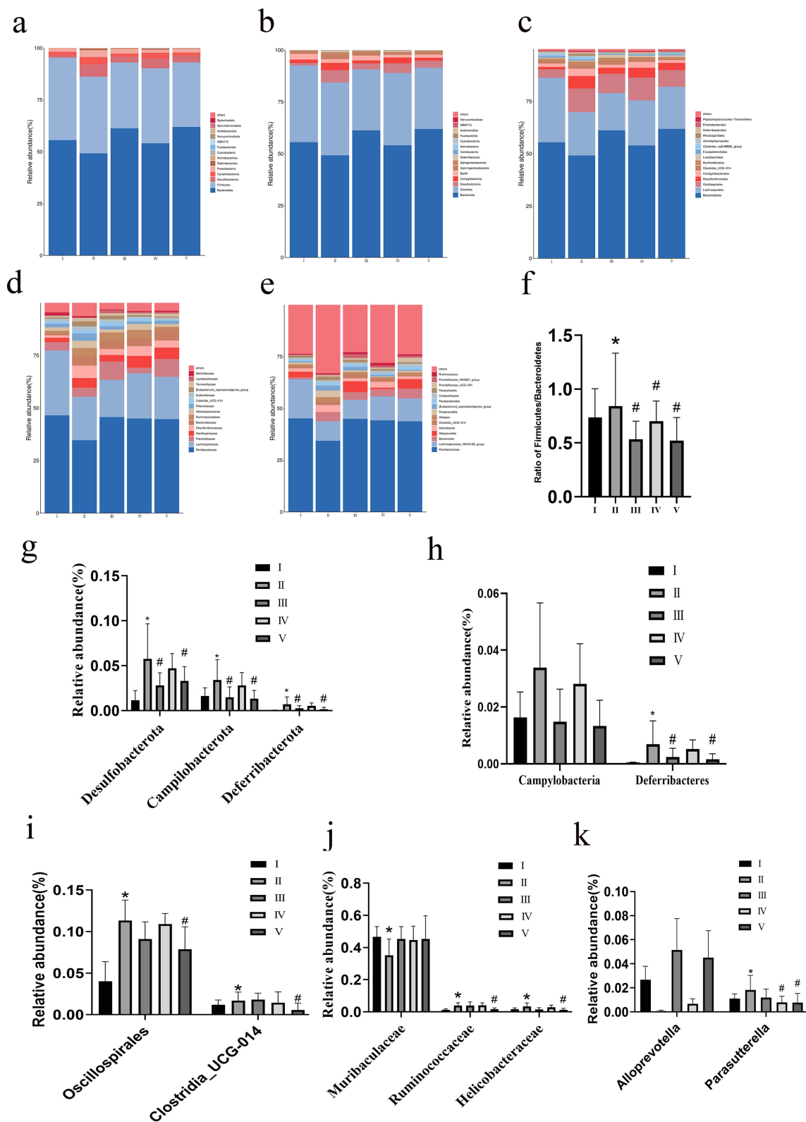
Figure 10 The effect of NC-CS/PT-NPs on gut microbiome composition of mice induced by HFD in different taxa. (a) Phylum. (b) Class. (c) Order. (d) Family. (e) Genus. (f) The ratio of Firmicutes / Bacteroidota . (g) Relative abundance of Phylum. (h) Relative abundance of Class. (i) Relative abundance of Order. (j) Relative abundance of Family. (k) Relative abundance of Genus. Compared with NCD group, * p < 0.05 ; compared with HFD group, # p < 0.05 . Notes: I NCD group. II: HFD group. III: Positive Control group. IV: NC-treated group. V NC-CS/PT-NPs treated group.
