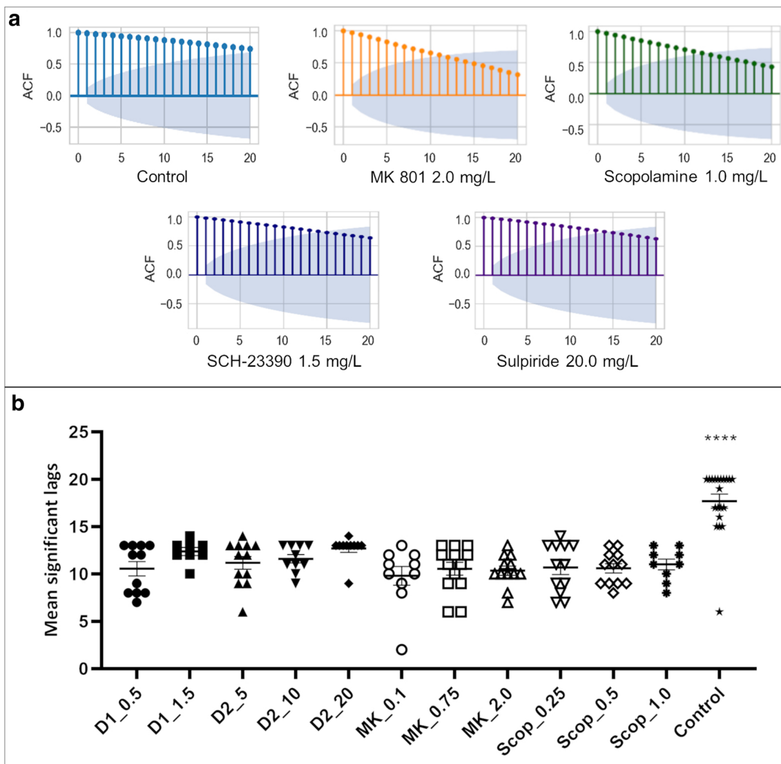
Fig. 8 (Top) ACF plot showing the first 20 lags of 250-lag plots. Each plot shows slow decay towards zero, with 18 lag points outside of the 95% C.I., depicted by the blue cone. ACF plots are individual animal responses in the FMP Y-maze and are therefore representative of the control group and drug treatment groups exposed to the highest concentration of antagonist for MK 801, scopolamine, SCH-23390 and
