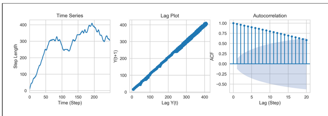
Fig. 4 Time series analysis of movement patterns of an individual zebrafish, zfl1, ( n=1 ), showing, from left to right, time series plot of the cumulative sum of step lengths for n=250 time points. Lag plot of data at lag-0 ( \omega(k) ) and lag-1 ( \omega(k+1) ) demonstrating a positive linear correlation. Autocorrelation function plot showing the first 20 lags of 250
