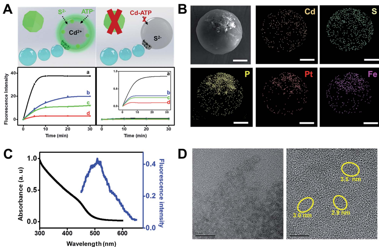
Fig. 3 (A) Schematic of the synthesis of CdS quantum dots using Janus microreactors with different configurations. The plots in the bottom part show the fluorescence intensity in the microreactor over time in (a) peroxide solution, (b) under magnetic stirring, (c) with microreactors containing \text{Fe}_3\text{O}_4 in peroxide solutions and (d) under static conditions. (B) SEM and EDX images showing the distribution of Cd, S, P, Pt and Fe in the microreactor. (C) Fluorescent emission and UV/VIS spectra of the as-synthesized CdS quantum dots. (D) HRTEM images of the CdS quantum dots. Scale bars, 5 \mu\text{m} (SEM) and 20 or 5 nm (HRTEM).
