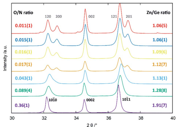
Fig. 3 XRD patterns in the region of 30^{\circ} – 40^{\circ} 2\theta as a function of Zn/Ge and O/N ratios. The hkl indices according to the hexagonal wurtzite-type structure (black, bottom) and the hkl indices according to the orthorhombic \beta -NaFeO 2 -type structure (grey, top) are given in the figure.
