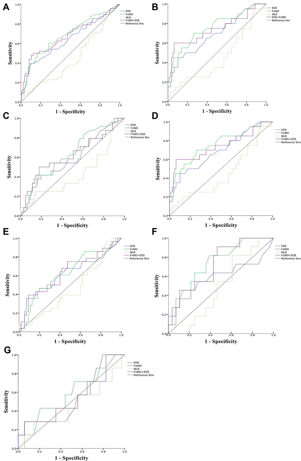
Figure 4 ROC curve for inflammatory markers for differentiating ACO from COPD.
