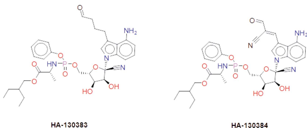
Fig. 9 The final suggested remdesivir analogs HA-130383 and HA-130384 of potential inhibitory activity against RdRp of SARS-CoV-2.
