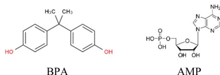
Scheme 1 Chemical structure of BPA and AMP.
