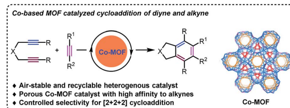
Scheme 1 Catalytic strategy for [2 + 2 + 2] cycloaddition in this work.
