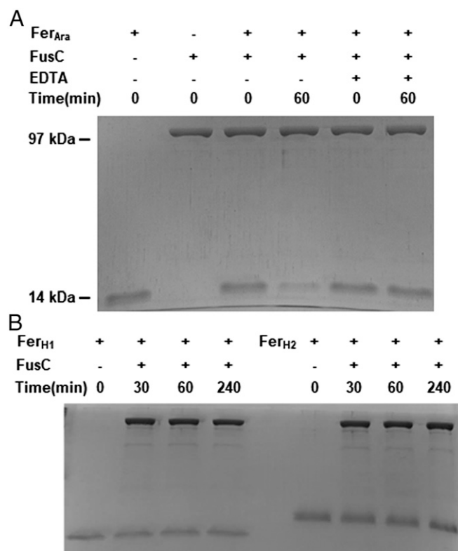
Fig. 1. FusC specifically cleaves plant ferredoxin. Purified His-tagged FusC (1 \mu M) was incubated in the presence or absence of either plant ferredoxin Fe_{Ara} (A) or human ferredoxin Fe_{H1} or Fe_{H2} (B) (10 \mu M) at room temperature in 50 mM Tris-HCl and 50 mM NaCl, pH 7.5. Reactions were quenched by the addition of SDS loading buffer, and proteins were resolved by 16% SDS-PAGE and stained with Coomassie blue. The position of the protein markers lysozyme (14 kDa) and phosphorylase b (97 kDa) are indicated, but the protein bands are not shown.
