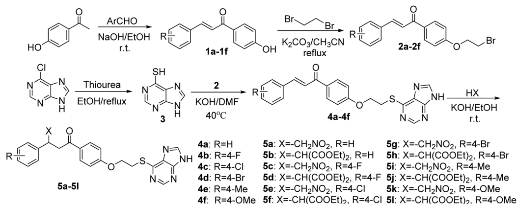
Scheme 1 The synthetic route of the target compounds 4a–4f and 5a–5l .
