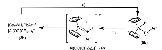
Scheme 8 (i): + Me NHC, toluene/o-DFB, rt, 3 h, – [ Me NHC–H][Al(OC(CF 3 ) 3 ) 4 ], (ii): + [H(Et 2 O) 2 ][Al(OC(CF 3 ) 3 ) 4 ], toluene/C 6 H 4 F 2 , rt, – 2 Et 2 O.
