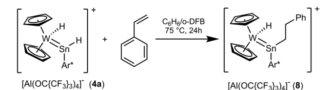
Scheme 7 Insertion of styrene into a Sn–H bond.
