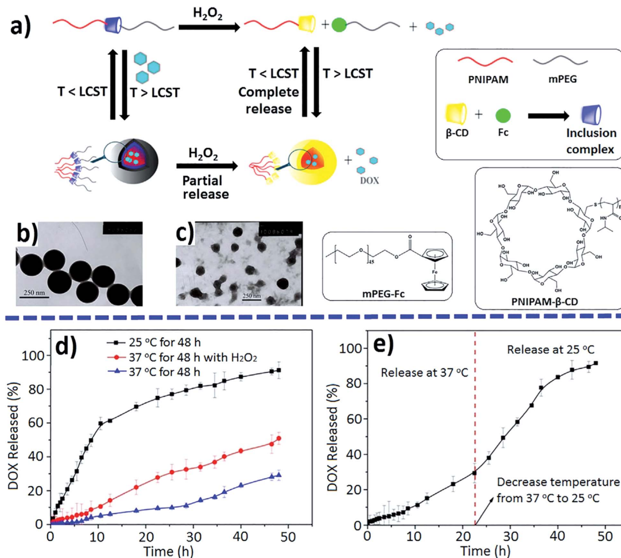
Fig. 36 Schematic dual-stimuli-responsive assembly and disassembly of mPEG-Fc/PNIPAM- \beta -CD micelles (a); TEM images before (b) and after oxidation (c) by \text{H}_2\text{O}_2 ; DOX-released profiles under single (d) or no stimulus and dual stimuli (e) [reprinted with permission from ref. 245. Copyright 2015, American Chemical Society].
