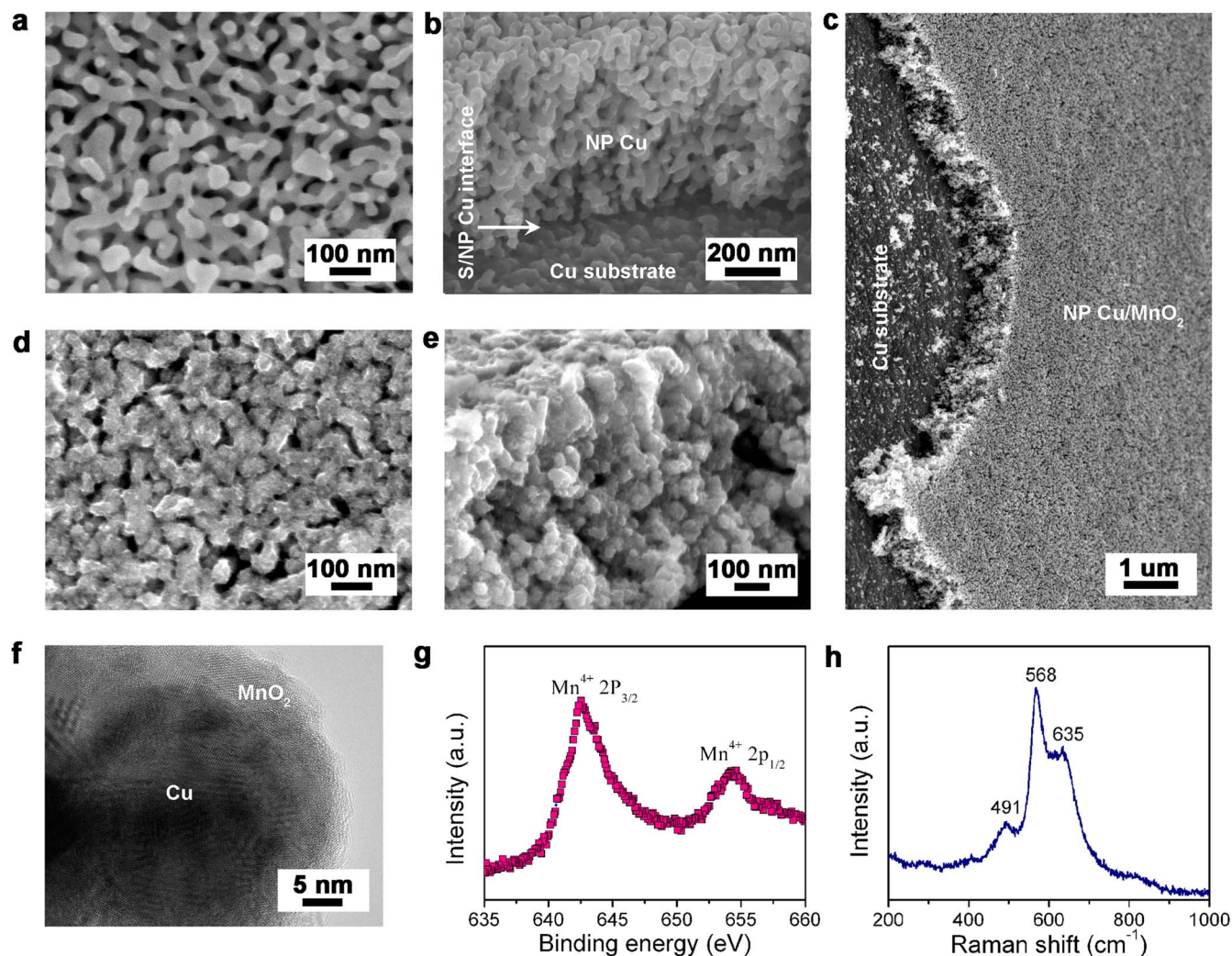
Figure 2 | Microstructure characterization. (a), (b), Top-view and cross-sectional SEM images of S/NP copper with a characteristic length of \sim 50 nm. (c), (d), (e), Low-magnification, top-view and cross-sectional SEM micrographs of S/NP Cu/MnO 2 after electroless plating. (f), Bright-field HRTEM image of the S/NP Cu/MnO 2 hybrid. The hybrid nanostructure can be identified by the contrast between the bright MnO 2 filler and the dark copper ligament. (g), XPS spectrum of Mn-2p orbit for the MnO 2 incorporated into S/NP Cu sheet. (h), Raman spectrum of S/NP Cu/MnO 2 hybrid bulk electrode.
