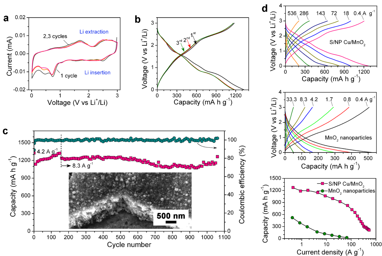
Figure 3 | Electrochemical performance. (a), CV curves at a scan rate of 0.2 \text{ mV s}^{-1} and, (b), galvanostatic charge/discharge profiles at the current rate of 0.8 \text{ A g}^{-1} for the initial three cycles of the S/NP Cu/MnO 2 electrode in the potential window of 0.01–3 V. (c), The reversible capacity retention and Coulombic efficiency of the S/NP Cu/MnO 2 hybrid bulk electrode during the first cycles at 4.2 \text{ A g}^{-1} followed by a higher current density of 8.3 \text{ A g}^{-1} . Inset: SEM micrograph of a S/NP Cu/MnO 2 hybrid bulk electrode after charge/discharge cycling. (d), Charge/discharge profiles of the S/NP Cu/MnO 2 electrode (top) and MnO 2 nanoparticles on Cu foil (middle) and the specific capacities of their constituent MnO 2 as a function of current density (bottom).
