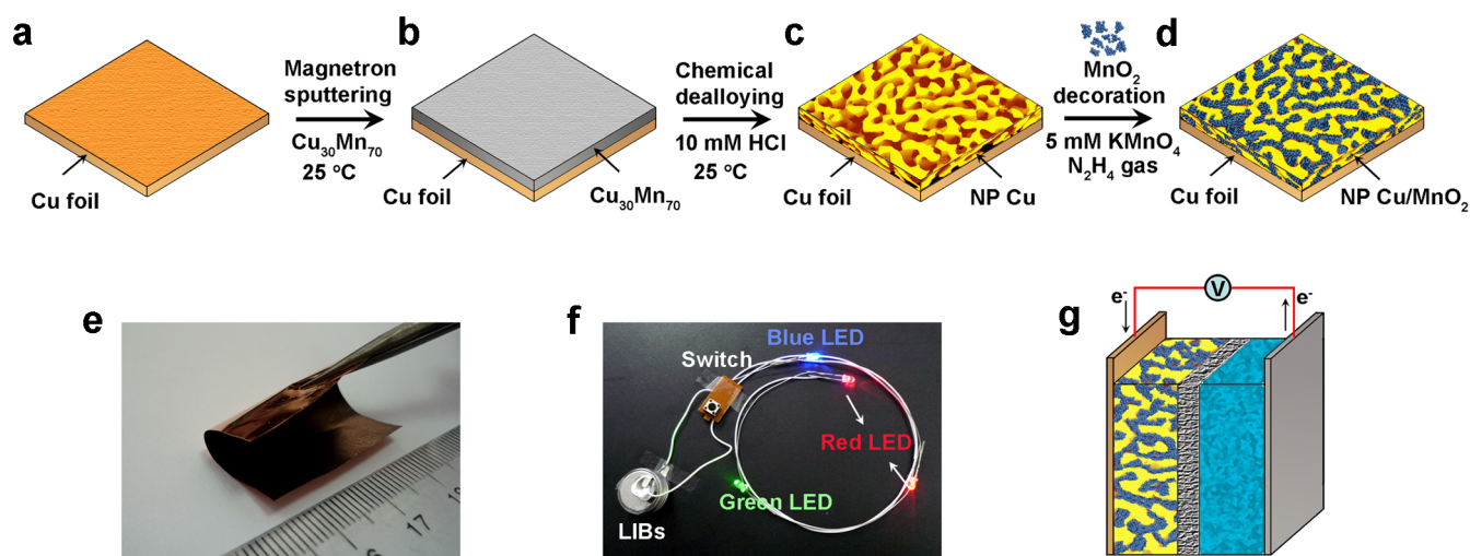
Figure 1 | Hybrid bulk electrodes with 3D nanoporosity for Li-ion batteries. Scheme showing the fabrication of seamlessly integrated S/NP Cu/MnO 2 bulk electrode: (a), Cleaned copper foil substrate; (b), Cu 30 Mn 70 alloy film deposited on the copper foil by magnetron sputtering; (c), Nanoporous Cu layer on the copper foil produced by chemical dealloying Cu 30 Mn 70 in diluted HCl solution; (d), Nanocrystalline MnO 2 directly grown onto S/NP Cu skeleton using electroless plating. (e), Photograph of a flexible S/NP Cu/MnO 2 hybrid bulk electrode being bend (2 × 3 cm 2 ). (f), Four batteries assembled with S/NP Cu/MnO 2 bulk electrodes power blue, red and green LEDs. (g), Schematic battery constructed with S/NP Cu/MnO 2 and lithium foil as electrodes, 1 M LiPF 6 in EC/EMC/DMC as electrolyte, and porous polymer as separator.
