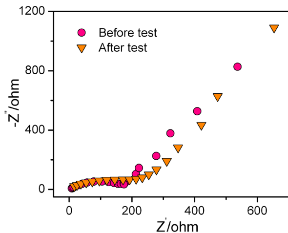
Figure 4 | Electrochemical impedance spectroscopy measurements. EIS spectra for the cell with S/NP Cu/MnO 2 electrode before and after the rate performance test.
