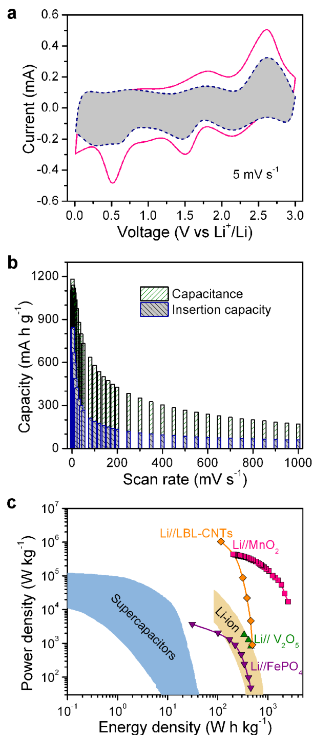
Figure 5 | Capacitance and Li-insertion/extraction contributions to charge storage/delivery and the Ragone plot. (a), Cyclic voltammetric responses for S/NP Cu/MnO 2 hybrid bulk electrode at a scan rate of 5 mV s -1 . The Li-insertion/extraction contribution is evaluated according to Eq. (1) and shown by the shaded region. (b), Capacitance and Li-insertion capacity for S/NP Cu/MnO 2 electrode as a function of scan rate. (c), The Ragone plot of the constituent MnO 2 nanoparticles in S/NP Cu/MnO 2 electrode, comparing with the energy and power densities of the active materials in the composites of CNT/FePO 4 3 , functionalized LBL-CNTs 14 , graphene/V 2 O 5 58 (only the active materials are included in the weight). The values of Li-ion nanoporous carbon/LiFePO 4 14,59 , LiNi 0.5 Mn 0.5 O 2 14,60 , and supercapacitive electrodes 11,14 are also included for comparison.
