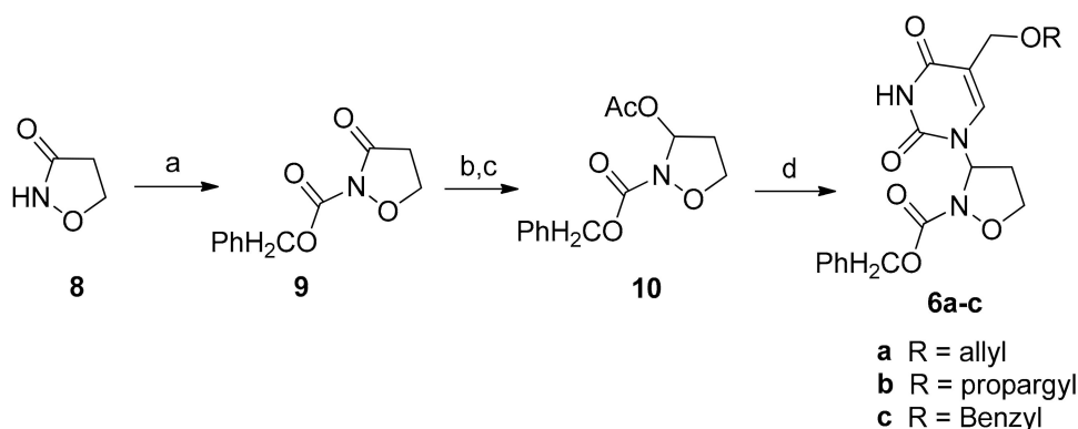
Scheme 1. Synthesis of 3'-pyrimidinyl isoxazolidines 6a–c : (a) ETA, \text{PhOCH}_2\text{C}(\text{O})\text{Cl} , DMF, room temperature; (b) \text{Cp}_2\text{Zr}(\text{H})\text{Cl} (4 equiv), THF, \text{SiO}_2 , 1 h, room temperature; (c) \text{Ac}_2\text{O} , ETA, DCM, room temperature, 6 h; (d) 5-substituted uracil 11a–c , BSA, TMSOTf, \text{CH}_3\text{CN} , r.t., 4 h.
