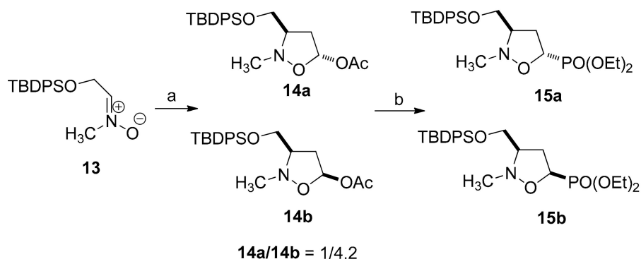
Scheme 3. Synthesis of phosphonated reverse homo- N,O -nucleosides 7a–d : (a) vinyl acetate, \text{CH}_2\text{Cl}_2 , 4 h, room temperature; (b) \text{P}(\text{OEt})_3 , \text{TiCl}_4 , \text{CH}_2\text{Cl}_2 , 4 h, -30^\circ\text{C} ; (c) TBAF, \text{CBr}_4 , THF, room temperature, 6 h; (d) nucleobase, \text{Cs}_2\text{CO}_3 , DMF, 95^\circ\text{C} , 4 h, room temperature.
