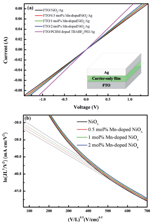
Fig. 1 (a) Linear sweep voltammetry curves of devices based on \text{TBABF}_4 -doped \text{PCBM}/\text{PEI} , un-doped and 0.5–2 mol% Mn-doped \text{NiO}_x ; (b) hole mobility of the un-doped and 0.5–2 mol% Mn-doped \text{NiO}_x versus electric field (V/L)^{0.5} .
