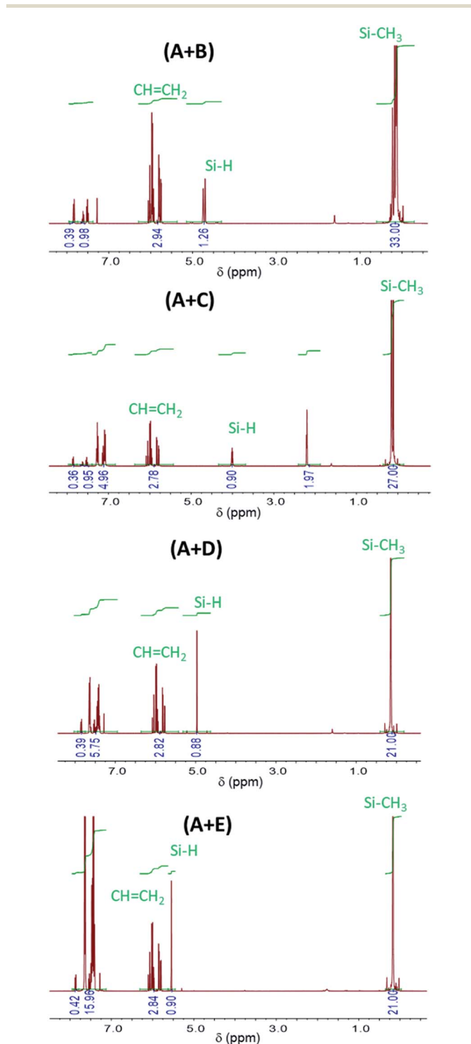
Fig. 1 1 H-NMR spectra of (A + B), (A + C), (A + D) and (A + E) formulations prior to UV irradiation ( t = 0 ).
