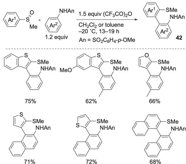
Scheme 21. Biaryl synthesis from aryl sulfoxides and sulfoanilides.
