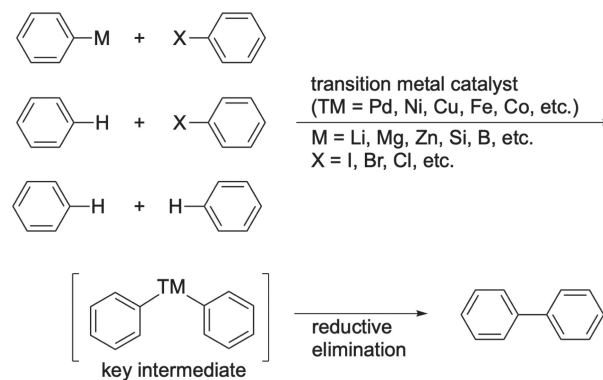
Scheme 1. Transition-metal-catalyzed coupling through reductive elimination.
