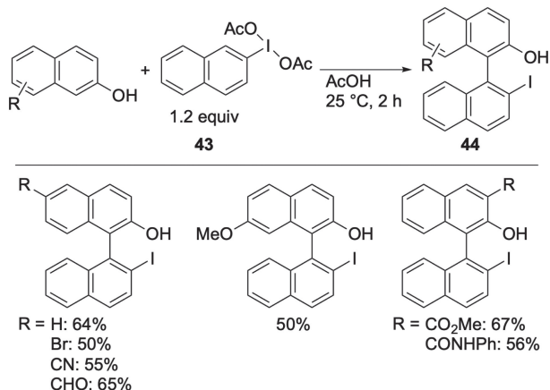
Scheme 22. Binaphthyl synthesis from 2-iodonaphthalene diacetate and 2-naphthols.
