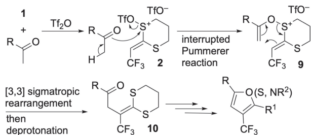
Scheme 6. \alpha -Functionalization of ketones for the synthesis of 3-trifluoromethylheteroles.
