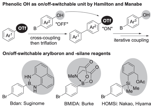
Fig. 4. On/off-switchable units for iterative cross-coupling.
