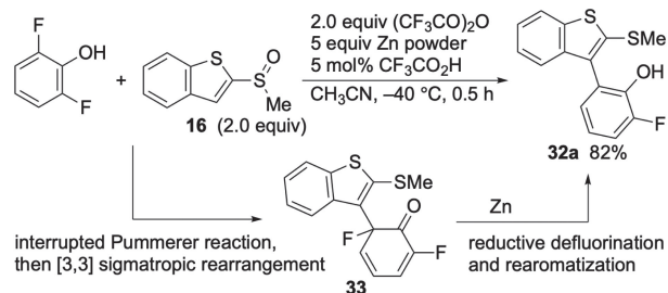
Scheme 15. Defluorinative synthesis of biaryls from 2,6-difluorophenol and benzothieryl sulfoxide with the aid of zinc as a reducing agent.
