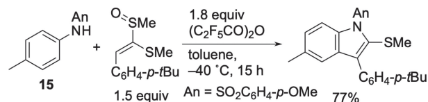
Scheme 8. Annulation between N -sulfonylaniline and KDM into indole.
