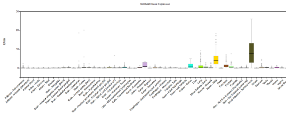
Figure 2. SLC6A20 expression patterns in different tissues extracted from GTEx portal
