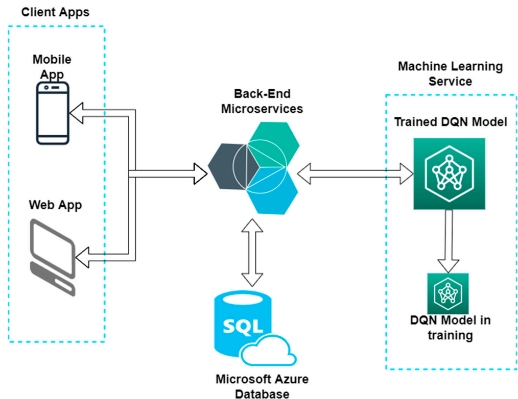
Figure 5. Architecture of the trained module.
