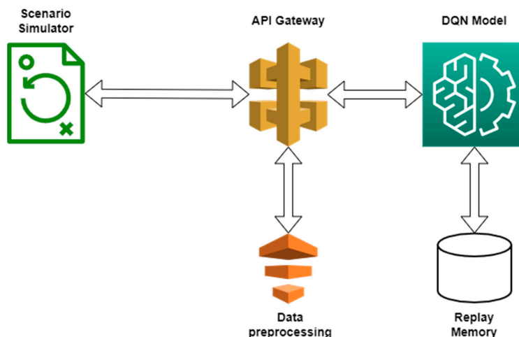
Figure 3. DQN Algorithm Workflow.
