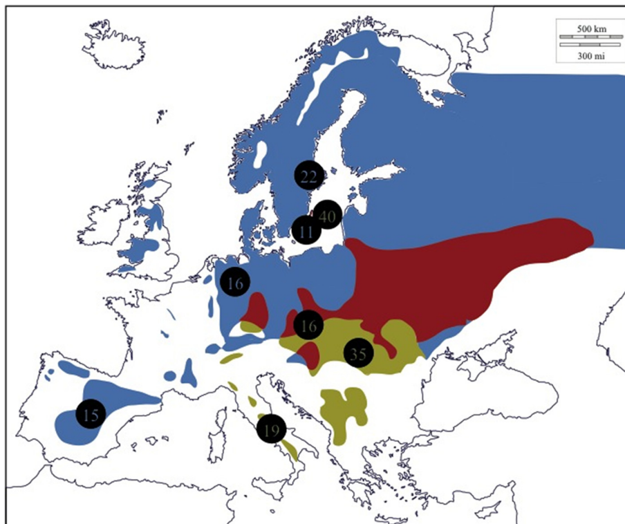
Figure 1 European breeding distribution ranges for the pied flycatcher ( Ficedula hypoleuca , light blue), the collared flycatcher ( Ficedula albicollis , green), and regions where both species occur together (red). Unreservedly redrawn and adapted from range maps in Cramp & Perrins [27]. Circles indicate sampling sites and the number of birds collected on each site is given within the circle. Numbers for pied flycatchers are in blue font and numbers for collared flycatchers are in green font.
