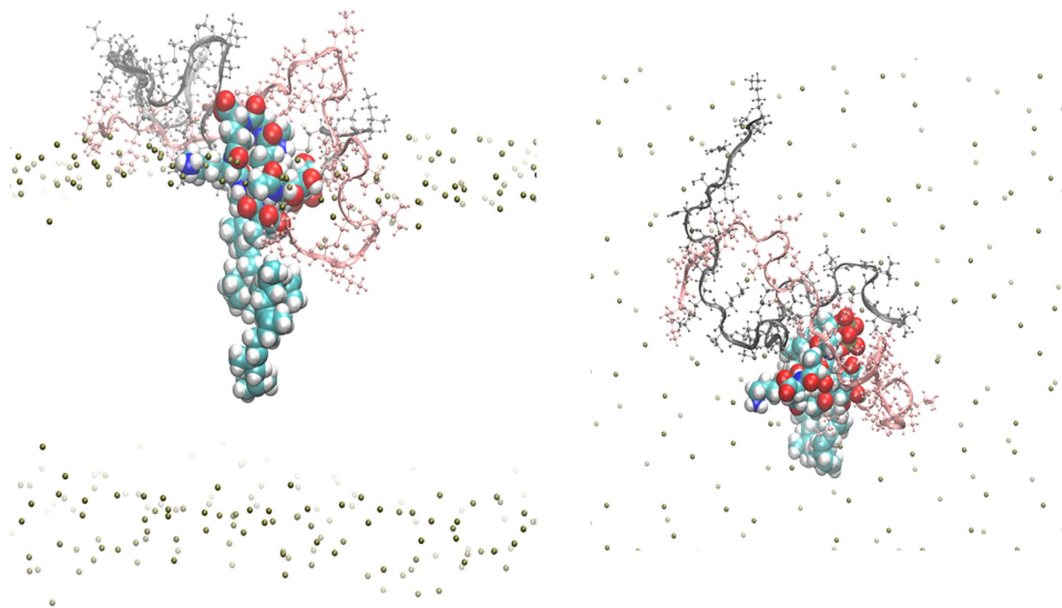
Figure 7. Trajectory snapshot from the MD simulation of the nisin 2 :lipid2 complex in a hydrated lipid membrane. Nisin 1 is displayed in grey carbon atoms and molecular surface, nisin 2 in pink carbon atoms and molecular surface, lipid II in cyan carbon atoms. Hydrogen bonds are displayed as green dashes. View of x-y plane.
