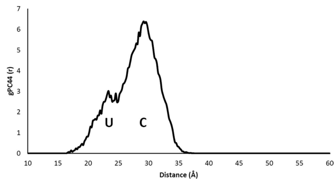
Figure 6. The radial distribution function of the lipid II tail terminus with respect to pyrophosphate in the hydrated bilayer simulation with two nisin molecules bound to the complex. The value of density set is 2 \times 10^{-6} , the number density of the single tail carbon atom in a sphere with 50 Å radius.
