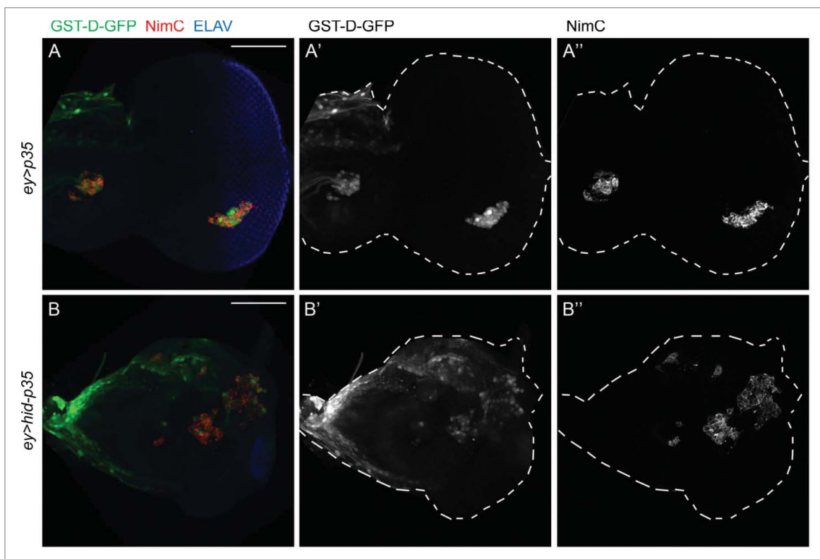
Figure 3. The redox reporter GST-D-GFP is expressed in hemocytes attached to both control and undead eye-antennal imaginal discs. Shown are eye-antennal imaginal discs of (A) ey-Gal4 UAS-p35 ( ey > p35 ; control) and (B) ey-Gal4 UAS-hid UAS-p35 ( ey > hid-p35 ; undead) genotype. Hemocytes are labeled using the NimC antibody (red in A, B; gray in A, "B"). GST-D-GFP is labeled in green in (A, B) and gray in (A', B'). NimC and GFP labeling overlap. Shown also in (A, B) is labeling with ELAV which marks photoreceptor neurons in the posterior part of the eye disc. ey-Gal4 is only expressed in the anterior portion of the eye disc, but when expressing hid and p35 , ey > Gal4 drives overgrowth of anterior tissue into the posterior part at the expense of photoreceptors. Scale bars, 100 \mu m.
