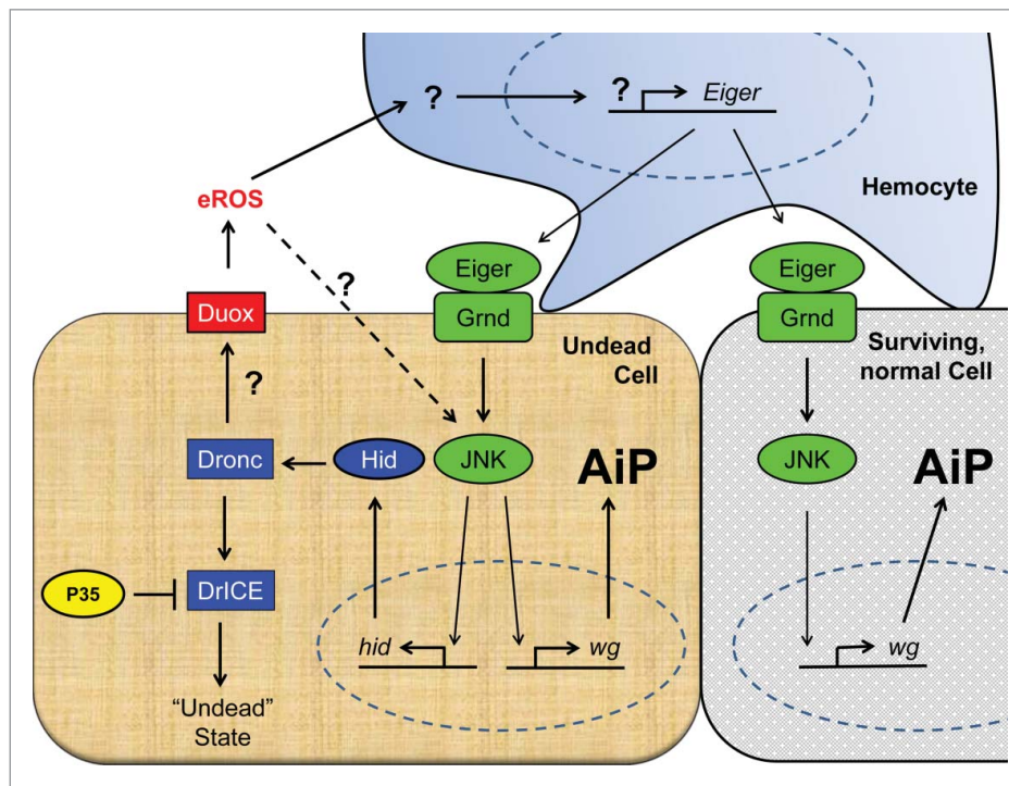
Figure 1. Schematic view of our current understanding of the cellular mechanisms of apoptosis-induced compensatory proliferation (AiP). Undead cells can be induced by co-expression of the pro-apoptotic gene hid and the effector caspase inhibitor p35 . Because P35 specifically inhibits the effector caspase DrICE (and Dcp-1; not shown), the initiator caspase Dronc cannot induce apoptosis (“undead” state), but remains active for apoptosis-independent functions. One of these functions is the activation of the transmembrane NADPH oxidase Duox, which generates extracellular ROS (eROS) such as superoxide and hydrogen peroxide. eROS activate and change the behavior of hemocytes to become proliferation-promoting. 3 This is accomplished through release of Eiger which activates the JNK pathway in undead and neighboring surviving cells. JNK stimulates the production of mitogens such as wingless ( wg ) (and dpp and spi ; not shown) for AiP. In undead cells, JNK also induces expression of hid which sets an amplification loop in motion. Factors involved in apoptosis are indicated in blue, in JNK activation in green and in production of ROS in red. Question marks indicate unknown mechanisms.
