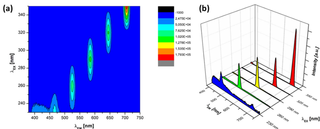
Fig. 10 (a) 3D excitation–emission spectra and (b) single PL emission spectra of the \text{SiO}_2/\text{ZnO} core–shell particles at various UV excitation wavelengths.
