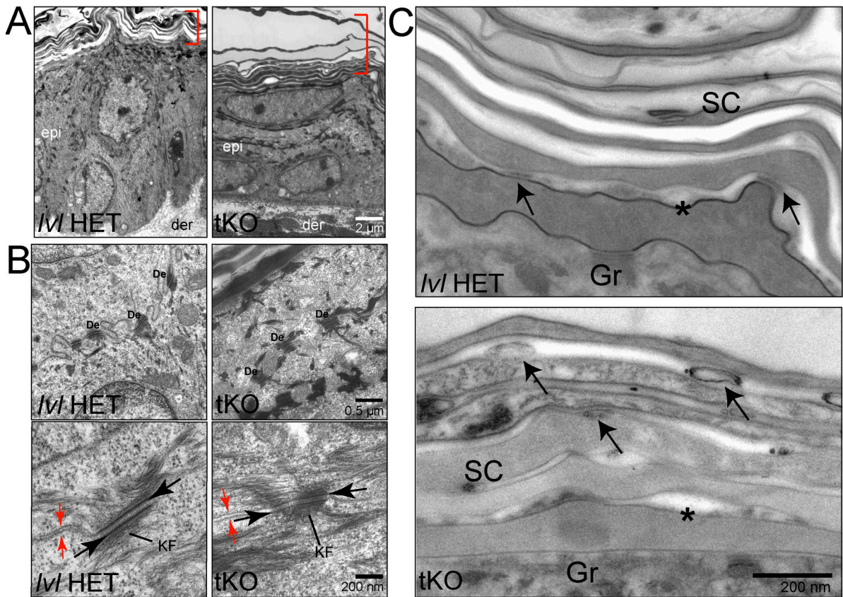
Figure 2. Ultrastructural changes in triple KO adult epidermis. (A) Low magnification views of sections of adult control ( involucrin ( l/l ) HET) and triple KO ( tKO ) dorsal epidermis. Red brackets mark cornified layers. Epi, epidermis; der, dermis. (B) Higher magnification images of desmosomes (De) and associated keratin intermediate filaments (KF). Triple KO desmosomes have a less distinct plaque (black arrows). Red arrows indicate adjacent cell membranes. (C) Higher magnification images of the granular layer (Gr)-stratum corneum (SC) interface and lower stratum corneum. Note altered morphology and prolonged retention of corneodesmosomes (black arrows) in the triple KO relative to the control. The CE is apparent as an electron dense line at the periphery of the corneocyte adjacent to the granular layer (asterisks). Note the decrease in electron density of this line in the triple KO.
