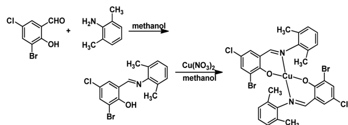
Scheme 1 The general synthetic routes for HL and the Cu(II) complex.
