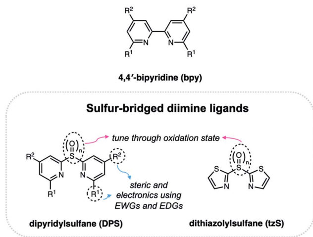
Fig. 15 Structure of 4,4'-bipyridine ligand (bpy) compared to sulfur-bridged diimine ligands based on dipirydylsulfane (DPS) and dithiazolylsulfane (tzS).
