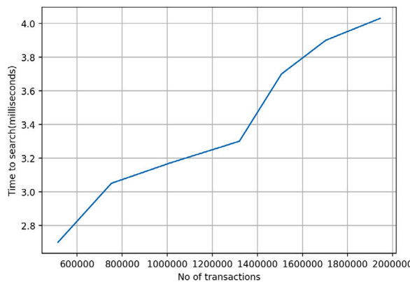
Fig. 15. Search performance of Connect platform.
