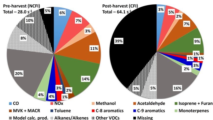
Figure 3. Pie charts showing the missing OH reactivities, and average contribution of measured OH reactants, estimated hydrocarbons and model calculated oxidation products to the total measured OH reactivity for (a) NCFI and (b) CFI periods.
