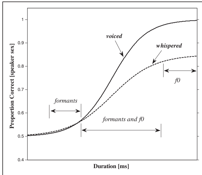
Figure 1. Hypothetical speaker-sex discrimination performance as a function of duration for voiced (solid line) and whispered (dashed line) speech. The general form of the psychometric functions is P(t) = \gamma + (1 - \gamma - \lambda)F(t) , where P(t) is the probability of correct discrimination of speaker sex at stimulus duration t , with guess rate \gamma (which in an m AFC task is 1/m , or 1/2 in our 2AFC task) which sets the lower asymptote representing chance performance, and with lapse rate \lambda which sets the upper asymptote representing ceiling performance. The function F is for convenience taken to be the logistic function [1 + \exp(-x)]^{-1} , which takes values between 0 and 1 for values of t , -\infty < t < \infty (see Treutwein & Strasburger, 1999). The bracketed region “formants” indicates durations where VTL-related information (the formants of speech) are the main cue to speaker sex discrimination, the region “ f_0 ” indicates durations where GPR-related information (voice pitch, as determined by f_0 ) is the main cue for discriminating speaker sex, and the region “formants and f_0 ” indicates durations where both formants and f_0 could contribute to speaker-sex discrimination. Proportion correct values on the y axis are for illustrative purposes only and axis durations are purposively left blank.
