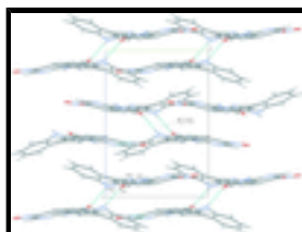
Fig. 4. View of the packing along [001] showing hydrogen bonds between the layers and the ring motif with descriptor R_2^2(10) .
