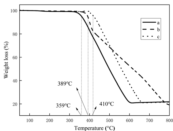
Fig. 1 The TGA curves of the three complexes: (a) (MPBFP) 2 Ir(detd), (b) (MPBFP) 2 Ir(tmd), and (c) (MPBFP) 2 Ir(acac).
