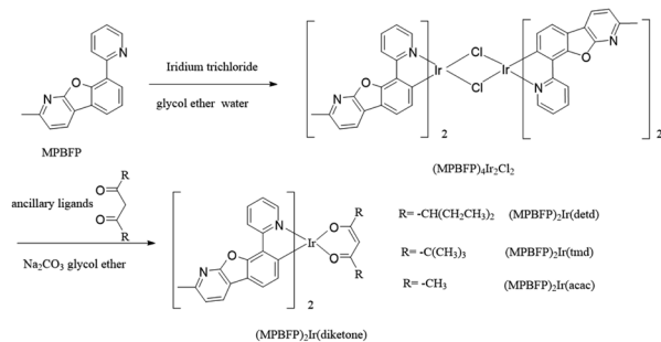
Scheme 2 Preparation of the chlorine-bridging dimer (MPBFP) 4 Ir 2 Cl 2 and three target metal complexes, namely (MPBFP) 2 Ir(detd), (MPBFP) 2 Ir(tmd) and (MPBFP) 2 Ir(acac).
