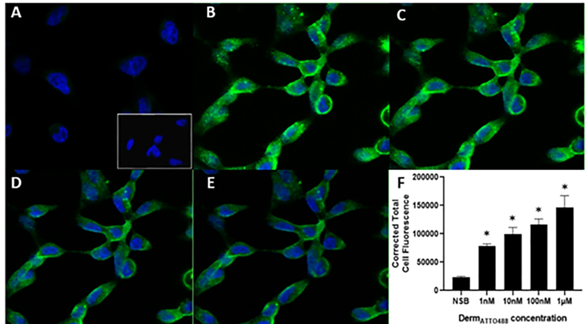
Fig 4. Concentration-dependent binding of Derm ATTO488 to MOP receptors expressed in HEK cells using confocal microscopy. Representative images of the binding of various concentrations (B: 1 μM, C: 100 nM, D: 10 nM and E: 1 nM). Nuclei are labelled (blue) with DAPI. Unlabelled (25 μM) Dermorphin blocked the binding of 1 μM Derm ATTO488 (16%) to the MOP receptors (A). Untransfected cells labelled 1 μM Derm ATTO488 are depicted in A-inset. Image F shows mean corrected total cell fluorescence ± SEM for n = 5 experiments and *p < 0.05 compared to NSB according to ANOVA followed by Dunnett's test for multiple comparison.
