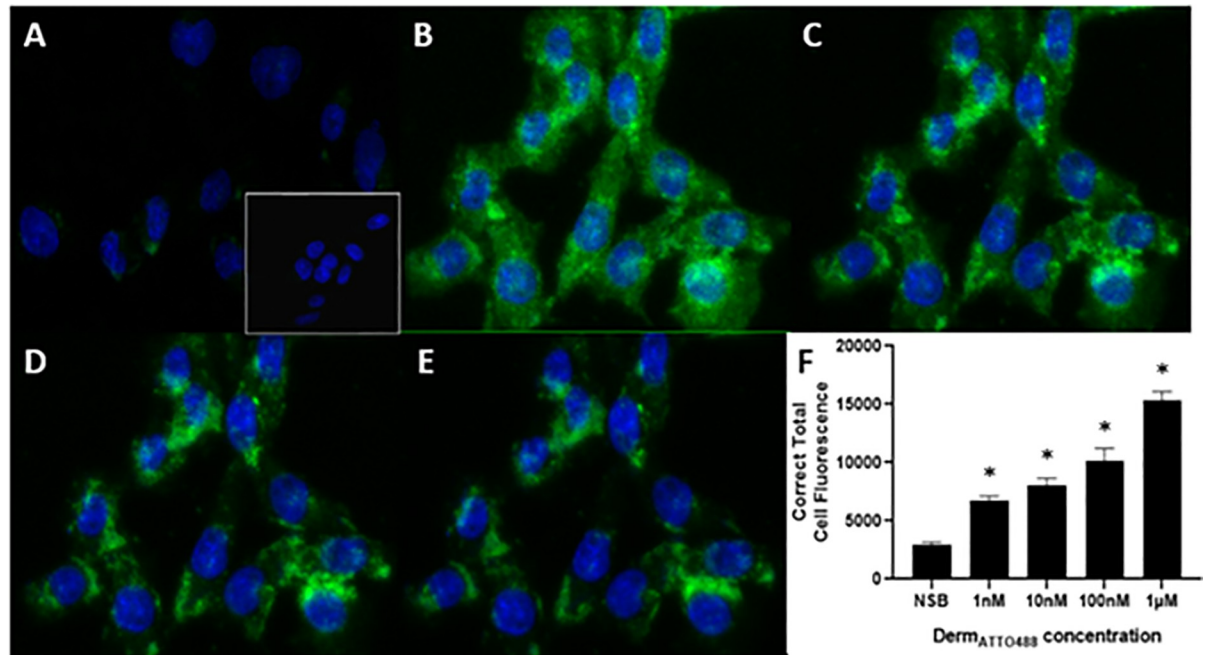
Fig 5. Concentration-dependent binding of Derm ATTO488 to the MOP receptors expressed in CHO cells using confocal microscopy. Representative images of the binding of various concentrations (B: 1 \mu M, C: 100 nM, D: 10 nM and E: 1 nM). Nuclei are labelled (blue) with DAPI. Unlabelled Dermorphin (25 \mu M) blocked the binding of 1 \mu M Derm ATTO488 (19%) to the MOP receptors (A). Untransfected cells labelled 1 \mu M Derm ATTO488 are depicted in A-inset. Image F shows mean corrected total cell fluorescence \pm SEM for n = 5 experiments and * p < 0.05 compared to NSB according to ANOVA followed by Dunnett's test for multiple comparison.
