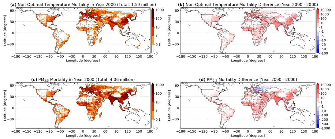
Supplementary Figure 2 Annual mortality for the year 2000 attributable to long-term exposure to non-optimal temperature (a) and to air pollution (c). The differences for the same results by the end of the century in the Shared Socio-economic Pathways SSP5-8.5 scenario are also presented (b) and (d).
