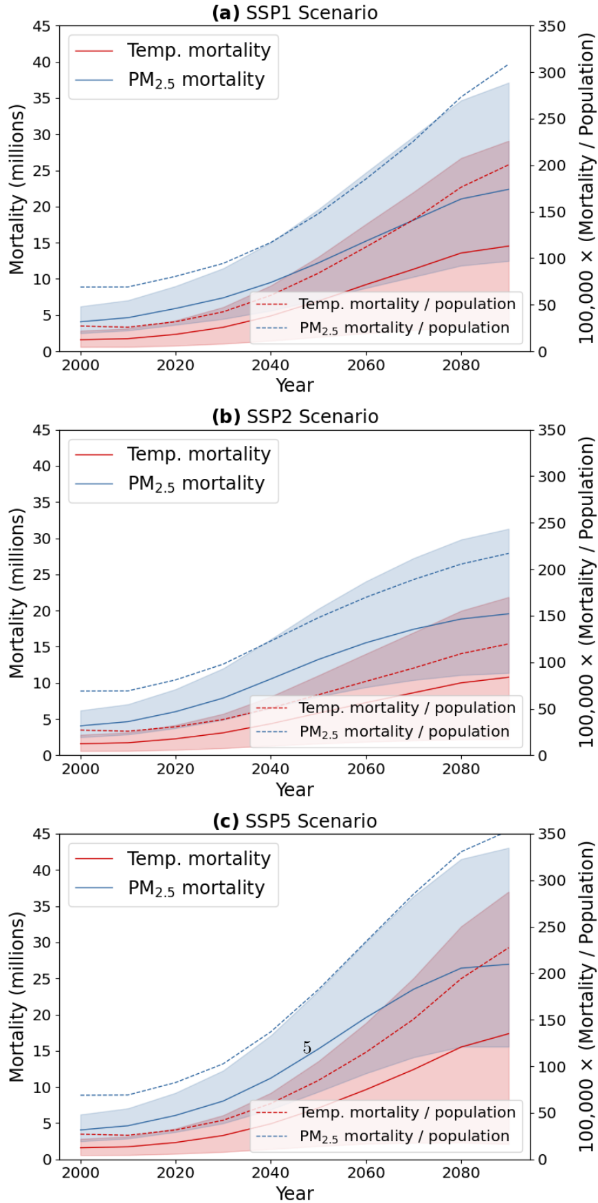
Supplementary Figure 6 Projected mortality as a function of time for the Shared Socio-economic Pathways SSP1-2.6 (a), SSP2-4.5 (b) and the SSP5-8.5 scenario (c). The solid curves, corresponding to the left vertical axes, show the total global mortality (in millions) due to air pollution and non-optimal temperature, with shading indicating the 95% confidence interval. The dashed curves, corresponding to the right axes, show the population-normalized mortality per 100,000 people.
