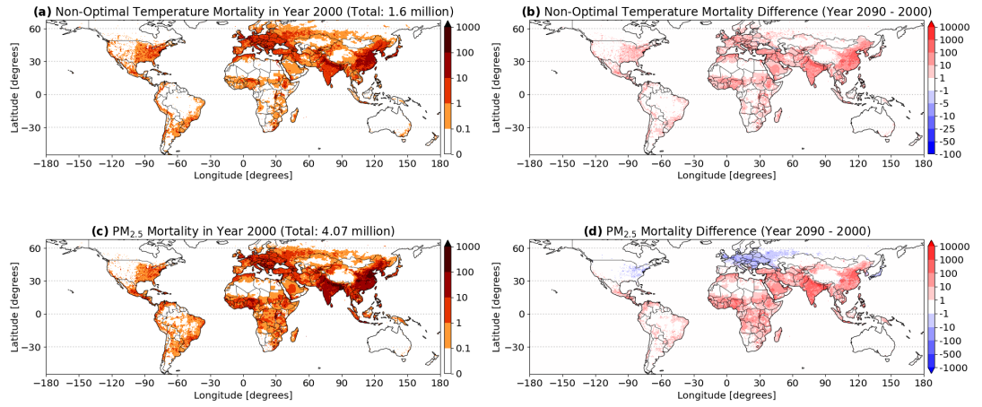
Supplementary Figure 1 Annual mortality for the year 2000 attributable to long-term exposure to non-optimal temperature (a) and to air pollution (c). The differences for the same results by the end of the century in the Shared Socio-economic Pathways SSP1-2.6 scenario are also presented (b) and (d).
