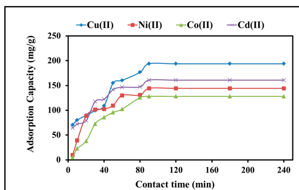
Figure 5. Effect of time of contact of heavy metal cations on the adsorption capacity upon mixing 0.3 g/L polyacrylamide functionalized Fe 3 O 4 nanoparticles with 150 mg/L metal cations solution at pH 6 and 25 °C.
