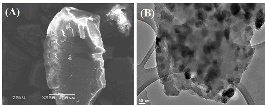
Figure 1. (A) SEM and (B) TEM of polyacrylamide functionalized Fe 3 O 4 nanoparticles.
