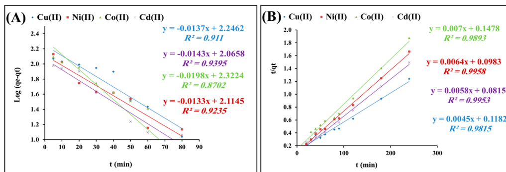
Figure 6. Pseudo-first-order (A) and pseudo-second-order; (B) of heavy metal adsorption tests upon mixing 0.3 g/L polyacrylamide functionalized \text{Fe}_3\text{O}_4 nanoparticles with 150 mg/L metal cations solution at pH 6 and 25 °C.
