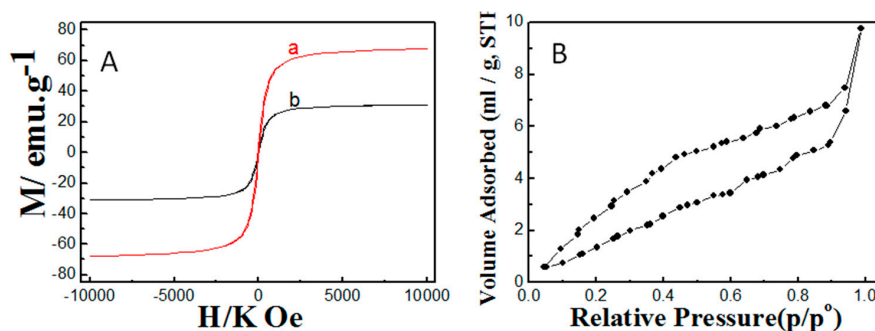
Figure 3. (A) Magnetic strength of (a) bare \text{Fe}_3\text{O}_4 and (b) polyacrylamide functionalized \text{Fe}_3\text{O}_4 ; (B) nitrogen sorption of polyacrylamide functionalized \text{Fe}_3\text{O}_4 nanoparticles.
