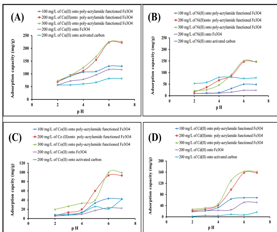
Figure 4. Effect of pH of (A) Cu(II); (B) Ni(II); (C) Co(II); and (D) Cd(II) on adsorption capacity upon mixing 0.5 g/L activated carbon with 200 mg/L of a metal cation solution, 0.5 g/L \text{Fe}_3\text{O}_4 nanoparticles, and 0.5 g/L polyacrylamide functionalized \text{Fe}_3\text{O}_4 nanoparticles with 100, 200, and 300 mg/L solutions of metal cations and 25 °C.
