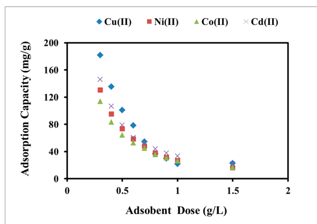
Figure 7. Effect of polyacrylamide functionalized \text{Fe}_3\text{O}_4 nanoparticles dose on the adsorption capacity of heavy metal cations at pH 6, contact time of 90 min, 140 mg/L of metal, and 25 °C.
