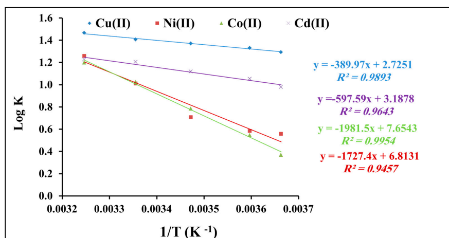
Figure 9. Thermodynamic factors for the adsorption of heavy metal cations onto polyacrylamide functionalized \text{Fe}_3\text{O}_4 nanoparticles.
