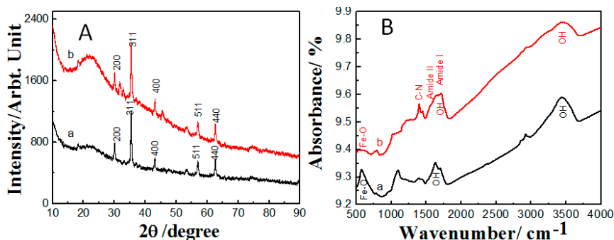
Figure 2. (A) XRD patterns and (B) FTIR spectra of (a) bare \text{Fe}_3\text{O}_4 and (b) polyacrylamide functionalized \text{Fe}_3\text{O}_4 nanoparticles.
