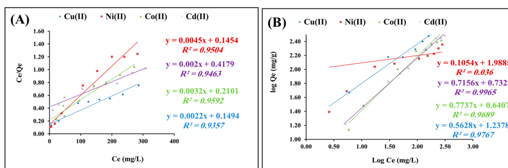
Figure 8. (A) Langmuir and (B) Freundlich isotherms for adsorption of heavy metal cations onto polyacrylamide functionalized Fe 3 O 4 nanoparticles.
