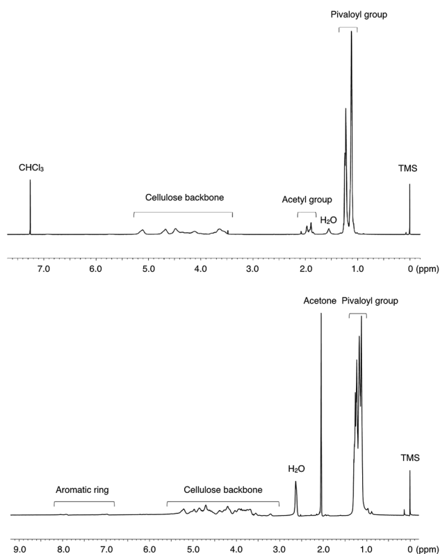
Fig. 2 ^1\text{H} NMR spectra of the resulting cellulose esters of Run 1 in \text{CDCl}_3 (upper) and Run 8 in \text{acetone-}d_6 (lower) measured at room temperature.
