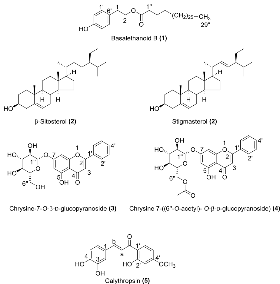
Figure 1. Chemical structures of compounds 1–5 isolated from the dichloromethane and methanol extracts of C. villosa stems.
