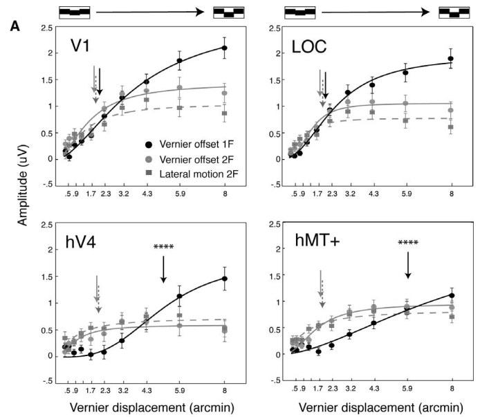
Figure 5. Comparison of sensitivity to relative position and motion in each ROI. SSVEP responses averaged across 15 participants as a function of Vernier displacement and lateral motion in different ROIs. The solid lines represent the first and second harmonic responses for Vernier onset/offset stimuli, and the dashed lines represent the second harmonic responses for lateral motion control stimuli. Both solid and dashed lines are fit by a generalized Naka-Rushton equation (see the Methods section and text). The arrows point to the semisaturation constant in each ROI. ****Paired t test between 1F and 2F of the Vernier response is significant at p < 0.0001 .
