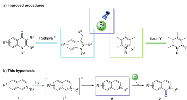
Scheme 1 The representative photocatalysis of oxidative approaches to the construction of N -substituted isoquinolin-1(2 H )-ones and 4-quinolones (a), and our hypothesis (b).
