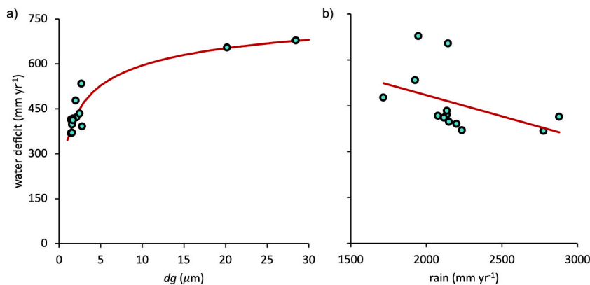
Fig. 25. Relationship between annual water deficit with soil texture (a) and annual rainfall (b). Soil texture is represented by d_g , which is the geometric mean diameter of the soil's three primary particle sizes, such that increasing d_g values indicate that soils have increasingly more sand and less clay [89].
