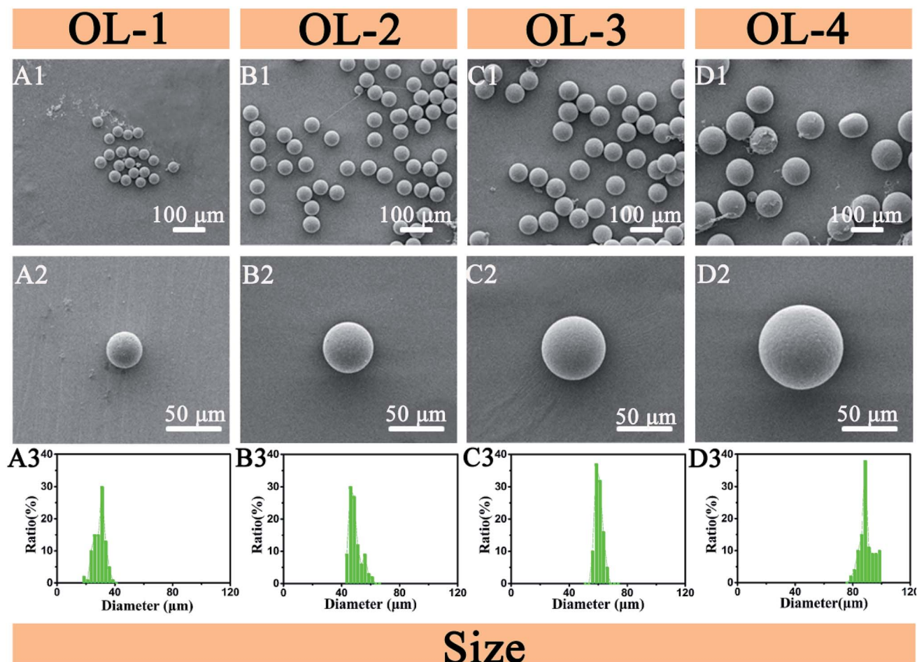
Fig. 3 SEM images (A1–D1 and A2–D2) and size distributions (A3–D3) of the four sizes of PLGA microparticles.
