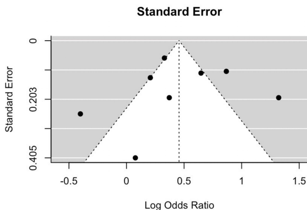
Figure 3 Funnel plot.
