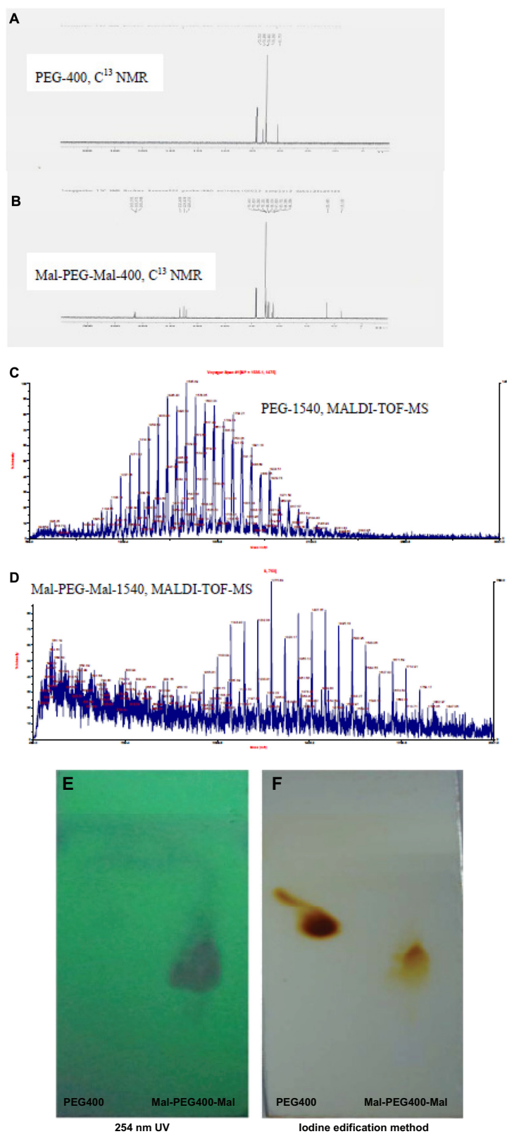
Figure S1 Data to examine the structures of Mal-PEG-Mal-400, Mal-PEG-Mal-1540. (A) PEG-400, C 13 NMR; (B) Mal-PEG-Mal-400, C 13 NMR; (C) PEG-1540, MALDI-TOF-MS; (D) Mal-PEG-Mal-1540, MALDI-TOF-MS; (E) 254 nm UV; (F) iodine edification method.
