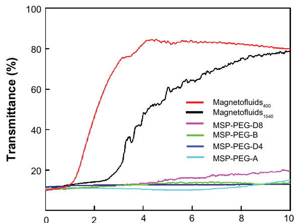
Figure S4 Suspension stability of some representative MSPs. Abbreviations: MSP, magnetic submicron particle; PEG, poly(ethylene glycol).
