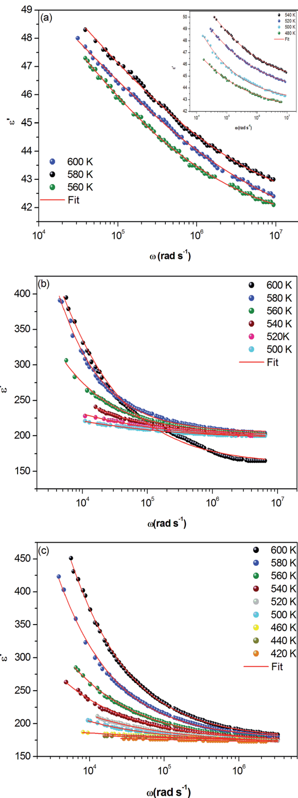
Fig. 8 (a, b and c) Frequency dependence of the real part of the dielectric constant, \varepsilon' at different temperatures for \alpha -NaCoPO 4 , \beta -NaCoPO 4 and \gamma -NaCoPO 4 respectively.
