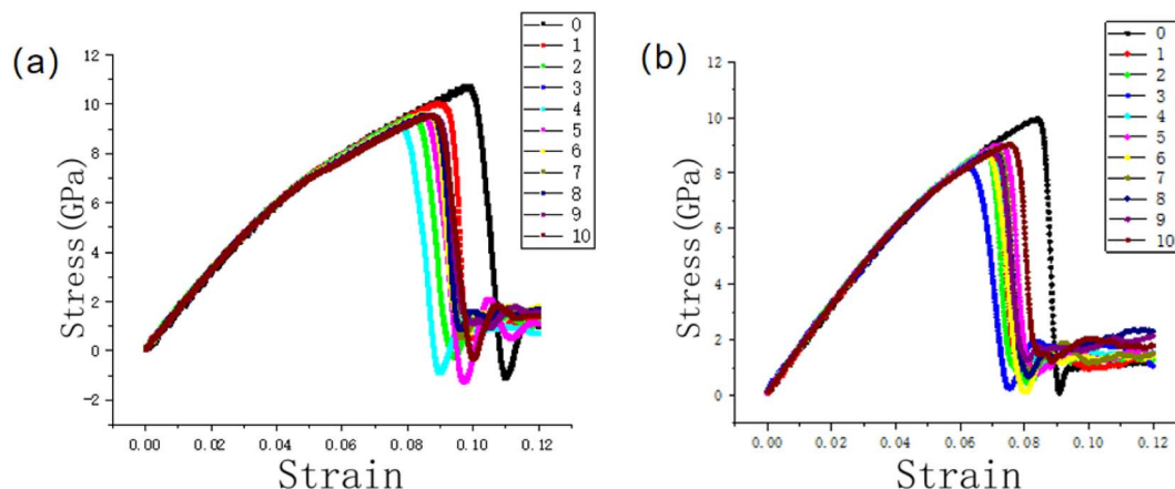
Fig. 2 Stress-strain curves of NW at 100 K (a) for Fe–Ni alloy NWs with 1.5% Ni and (b) for Fe–Ni alloy NWs with 8.5% Ni. The color curves correspond to the NW with the different number of CTB layers.
