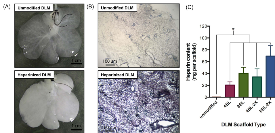
Figure 3. Characterization of heparinized DLM scaffolds. (A) Macroscopic images (B) Histological toluidine blue staining of unmodified and 4BL–2X heparinized DLM scaffolds. (C) Quantification of heparin content of the scaffolds after LbL deposition. Scale bars, (A) 1 cm, (B) 100 \mu m. * p = 0.0161
