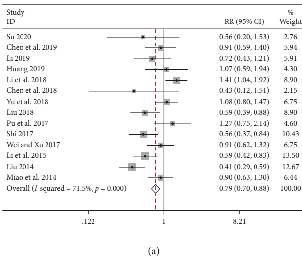
FIGURE 8: Meta-analysis showing a significant reduction in the platelet toxicity in the experimental group compared with that of the control group. (a) Meta-analysis of platelet toxicity in included studies. (b, c) The impact of the literature on heterogeneity by the L'Abbe plot and Galbraith plot. (d) The sensitivity analysis of the eight included articles.
