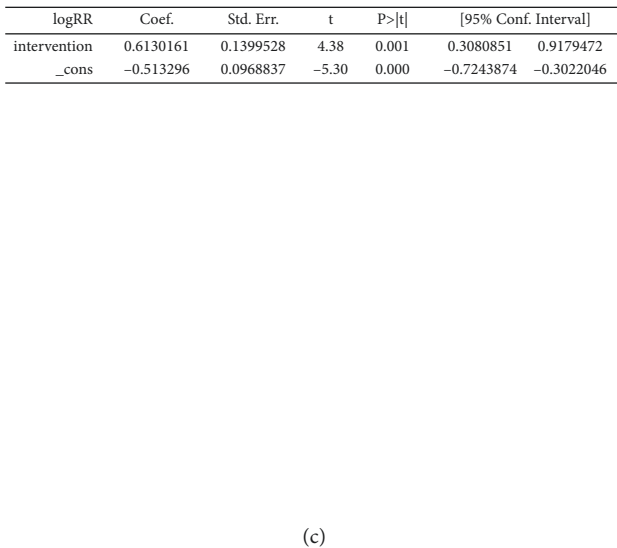
FIGURE 9: (a) Meta-analysis of vomiting response in included studies. (b, c) The results of the meta-regression analysis. (d) The subgroup study of vomiting toxicity.
