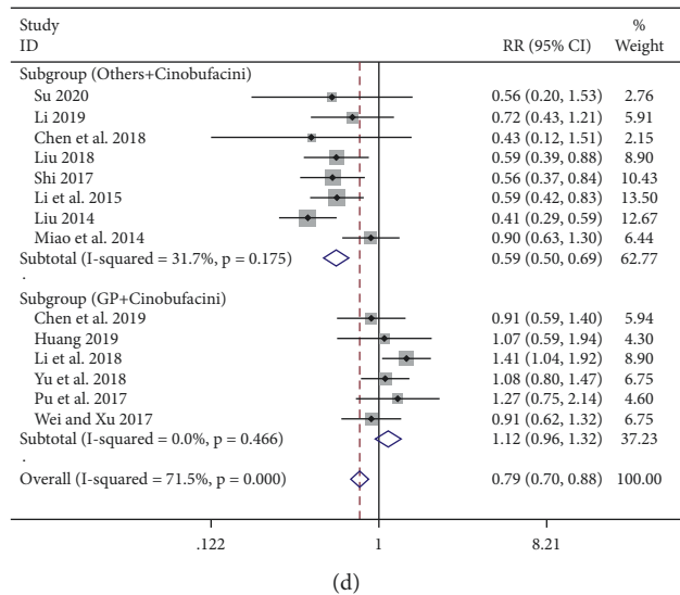
FIGURE 9: (a) Meta-analysis of vomiting response in included studies. (b, c) The results of the meta-regression analysis. (d) The subgroup study of vomiting toxicity.
