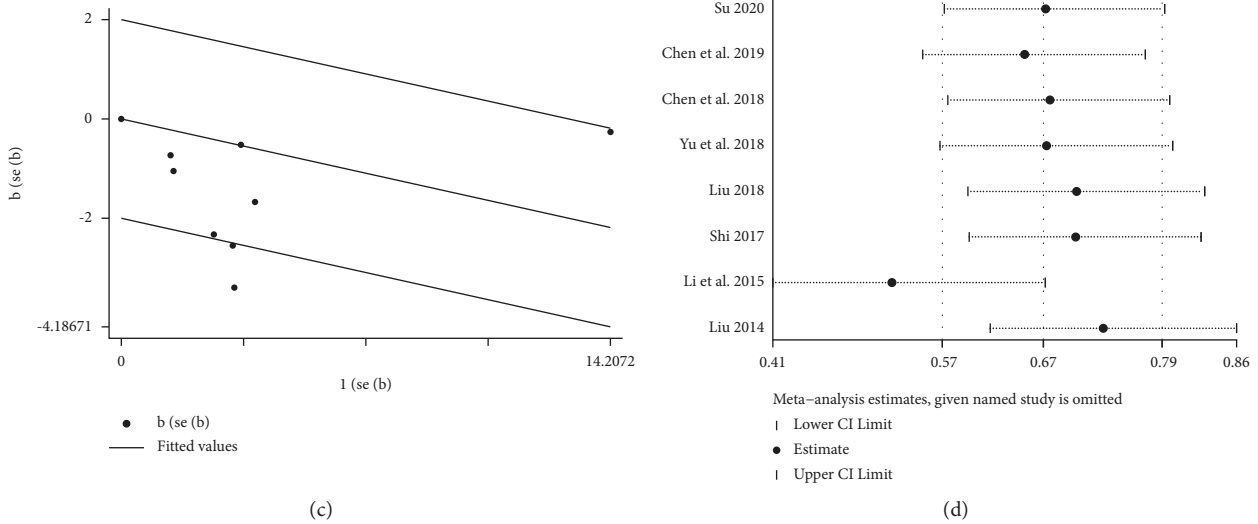
FIGURE 8: Meta-analysis showing a significant reduction in the platelet toxicity in the experimental group compared with that of the control group. (a) Meta-analysis of platelet toxicity in included studies. (b, c) The impact of the literature on heterogeneity by the L'Abbe plot and Galbraith plot. (d) The sensitivity analysis of the eight included articles.
