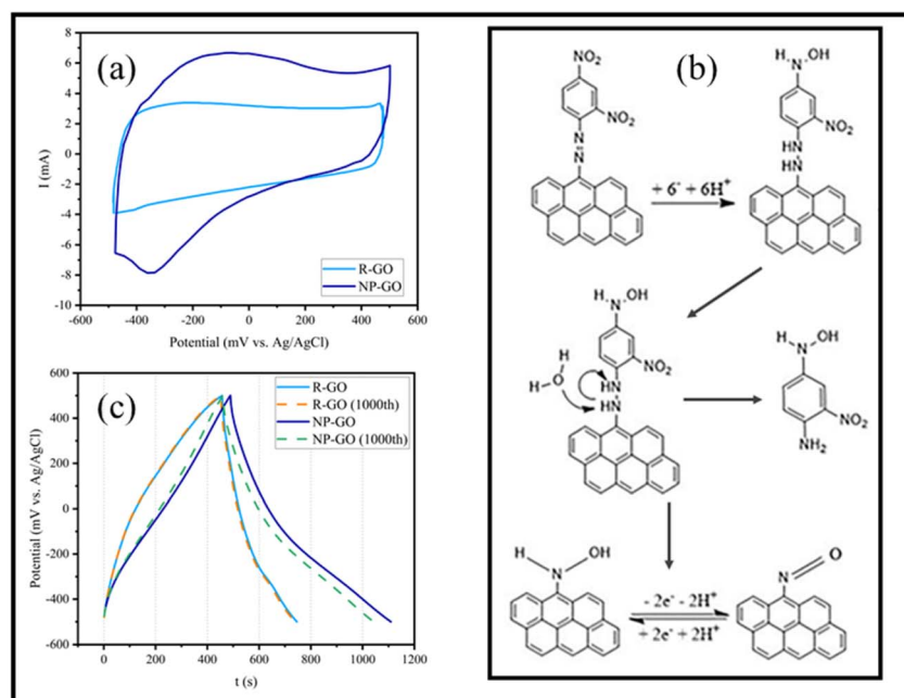
Fig. 7 (a) Cyclic voltammetry of electrodes made of R-GO and NP-GO at the scan rate of 5 \text{ mV s}^{-1} , (b) the mechanism of the reduction of 2,4-dinitrophenylhydrazone presented on the surface of NP-GO in an aqueous environment and the redox reaction of the nitroso group, (c) First and 1000th galvanostatic charge/discharge of R-GO and NP-GO at 0.5 \text{ A g}^{-1} .
