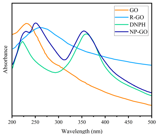
Fig. 3 UV spectra of GO, R-GO, DNPB, and NP-GO.
