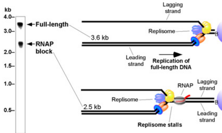
Figure 1 The replisome is impeded by a head-on RNAP.
